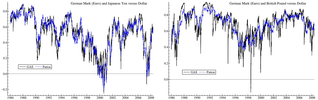
Figure 1: A copula illustration: comparisons of the correlation parameter estimates for the GAS and Patton models in (24)–(25). The data are the marginal AR-GARCH transforms of log exchange rates for the German Mark-US dollar and Japanese Yen-US dollar (left panel) and for the German Mark-US dollar and British Pound-US dollar (right panel). The sample period is January 1986–August 2008.
