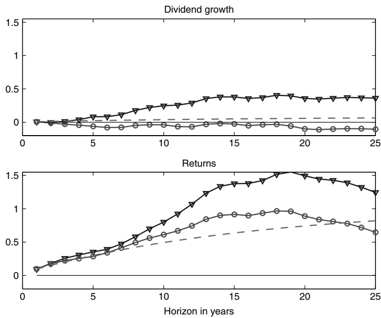
Figure 7 Regression forecasts of discounted dividend growth \sum_{j=1}^k \rho^{j-1} \Delta d_{t+j} (top) and returns \sum_{j=1}^k \rho^{j-1} r_{t+j} (bottom) on the log dividend yield d_t - p_t , as a function of the horizon k . Triangles are direct estimates: I form the weighted long-horizon returns and run them on dividend yields—for example, \beta\left(\sum_{j=1}^k \rho^{j-1} \Delta d_{t+j}, d_t - p_t\right) . Circles sum individual estimates: I run dividend growth and return at year t + j on the dividend yield at t and then sum up the coefficients—for example, \sum_{j=1}^k \rho^{j-1} \beta(\Delta d_{t+j}, d_t - p_t) . The dashed lines are the long-run coefficients implied by the VAR—for example, \sum_{j=1}^k \rho^{j-1} \phi^{j-1} b_d .
