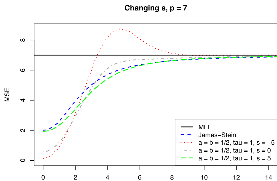
Figure 3: Mean-squared error as a function of \|\beta\|^2 for p = 7 and various cases of the hypergeometric inverted-beta hyperparameters.
