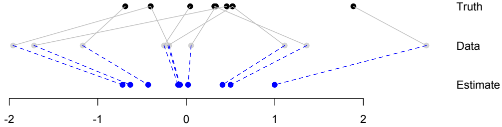
Figure 1: Ten true means drawn from a standard normal distribution; data from these means under standard normal noise; shrinkage estimates under the half-Cauchy prior for \lambda .
