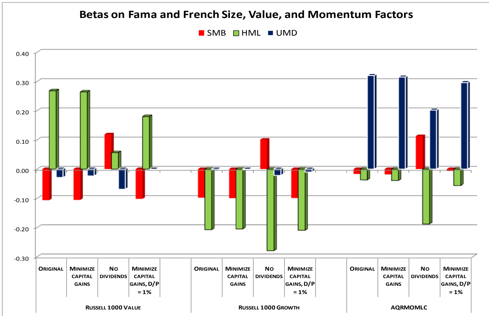
Figure 4: Fama-French Four Factor Exposure of Tax managed and Tax Unaware Equity Style Portfolios
