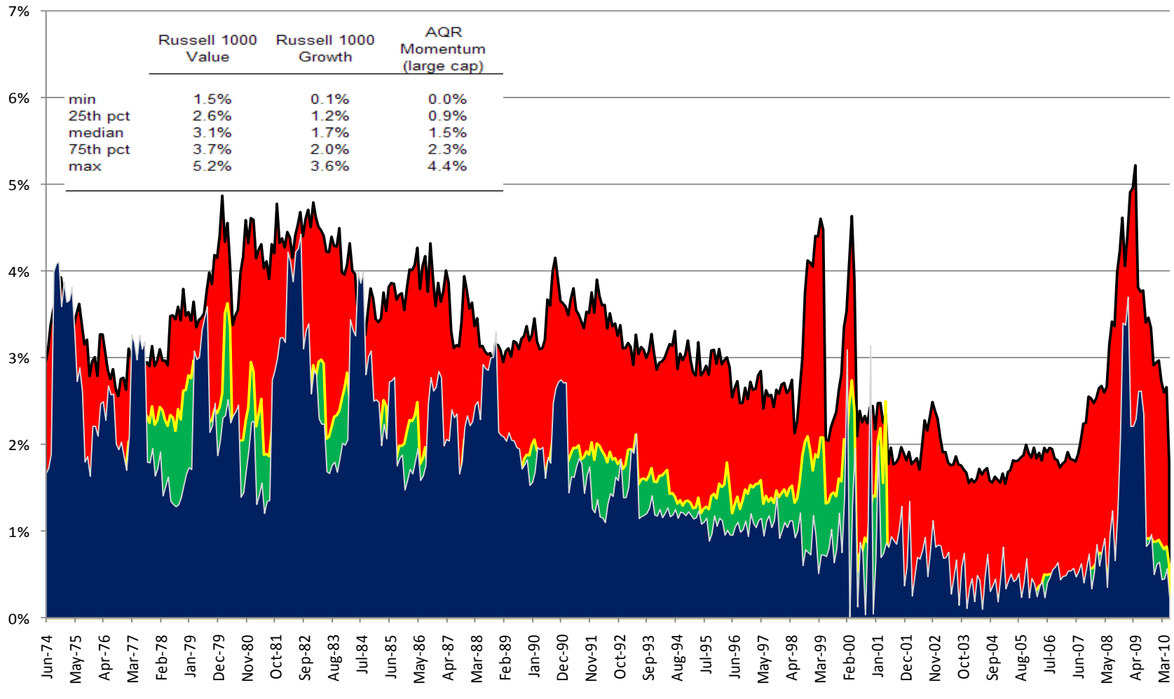
Figure 3: Tracking Error of Tax managed Portfolio to Original Index
