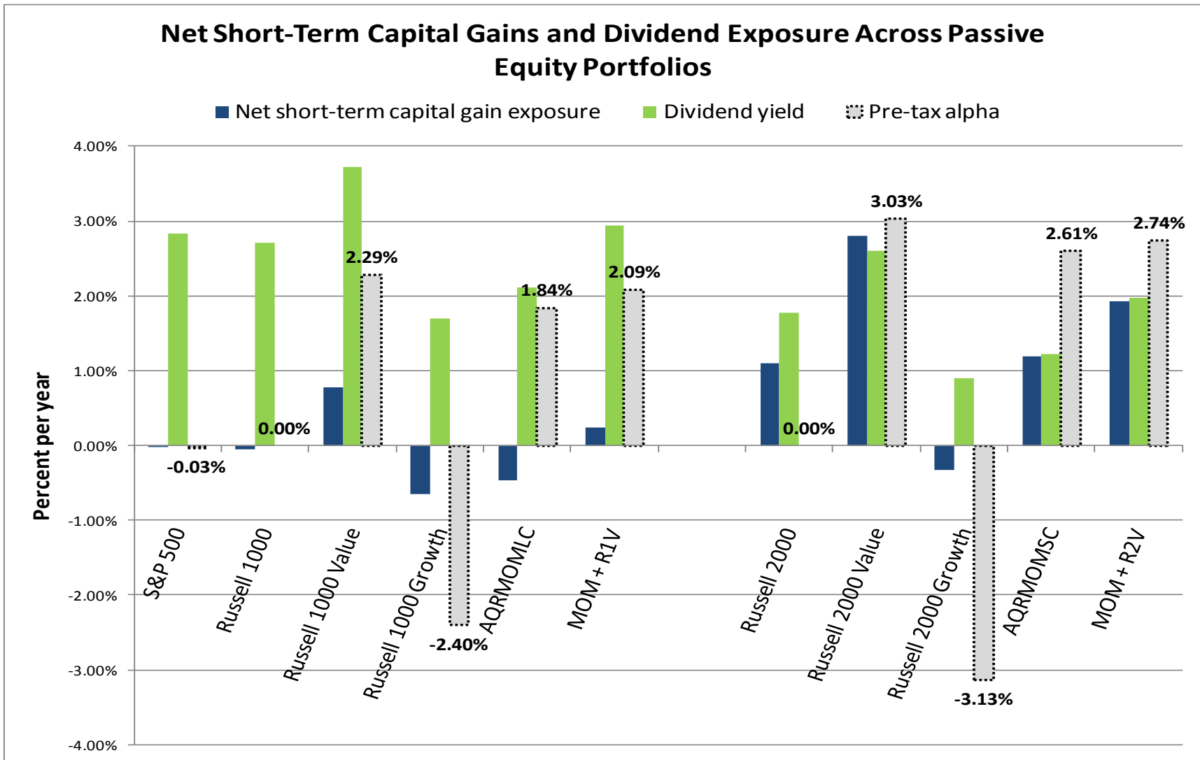
Figure 1: Net Short-Term Capital Gains, Dividend Exposure and Pre-tax Alphas Across Equity Styles
