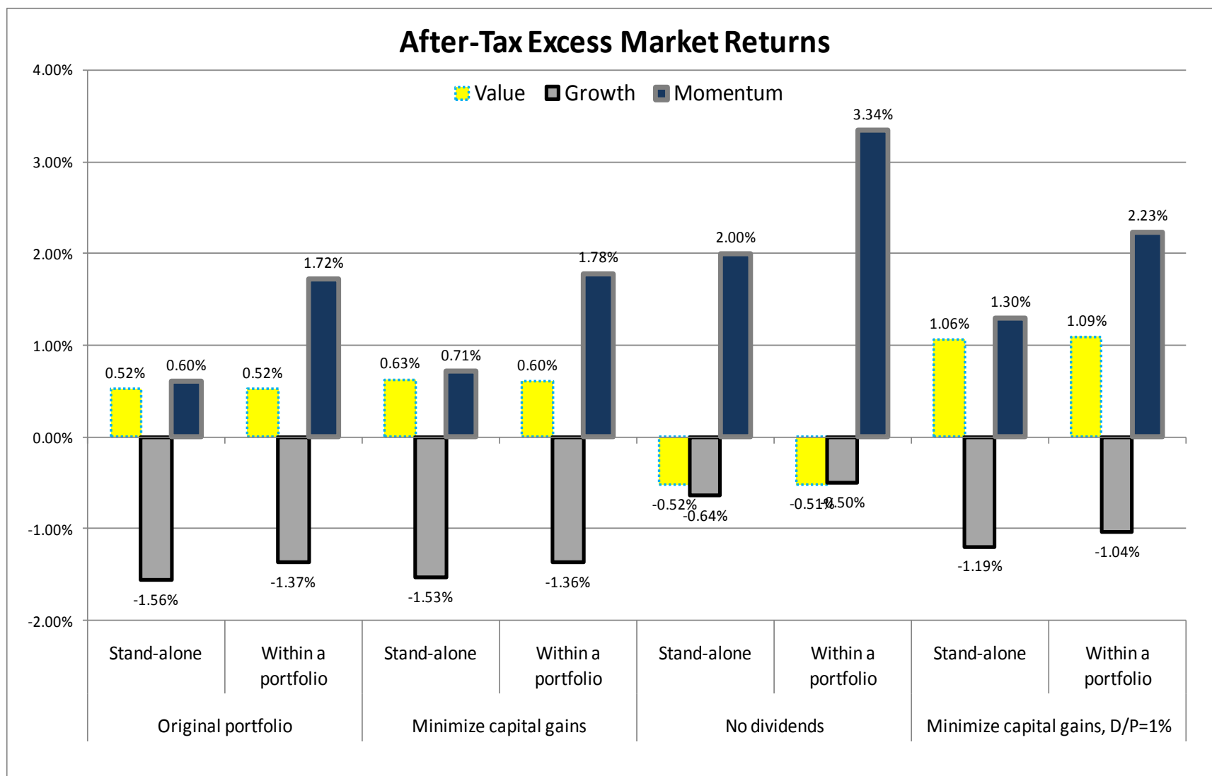
Figure 5: After-Tax Excess Market Returns of value, growth, and momentum
