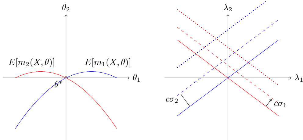
Figure 4.1: Moment inequalities (left) and linearized constraints (right)
