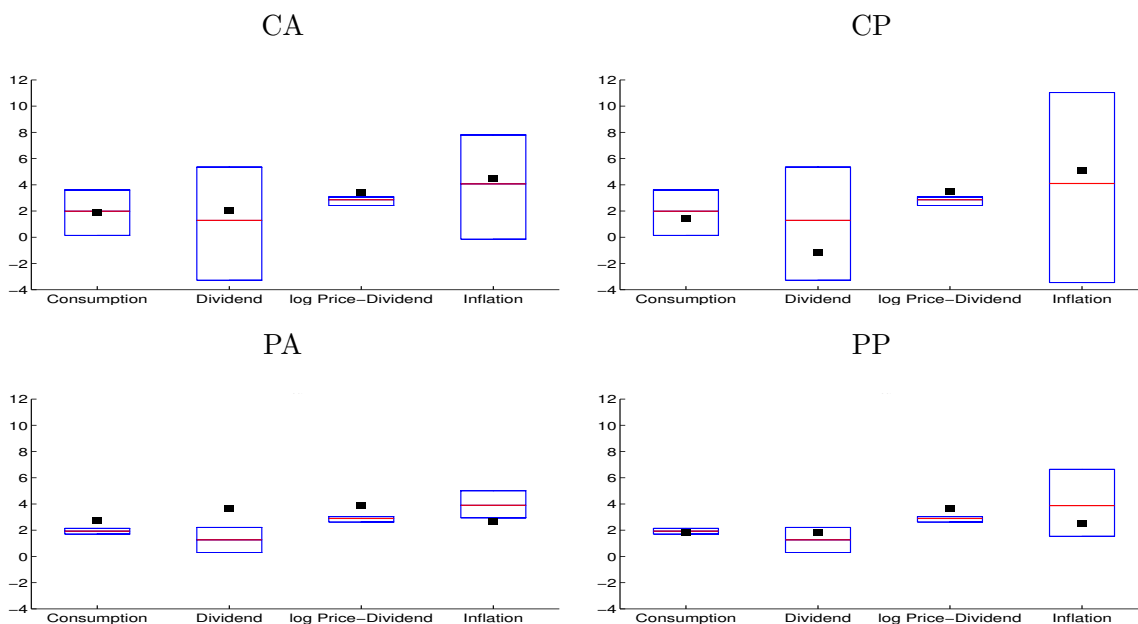
Figure A-3: Model-Generated Unconditional Mean
