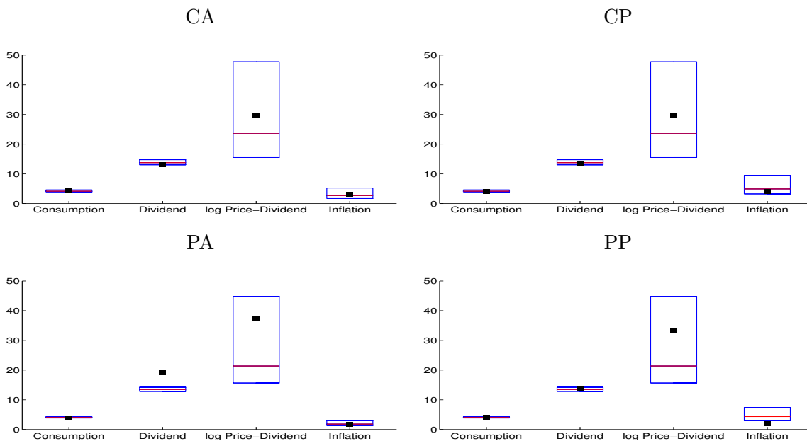
Figure A-4: Model-Generated Unconditional Standard Deviation
