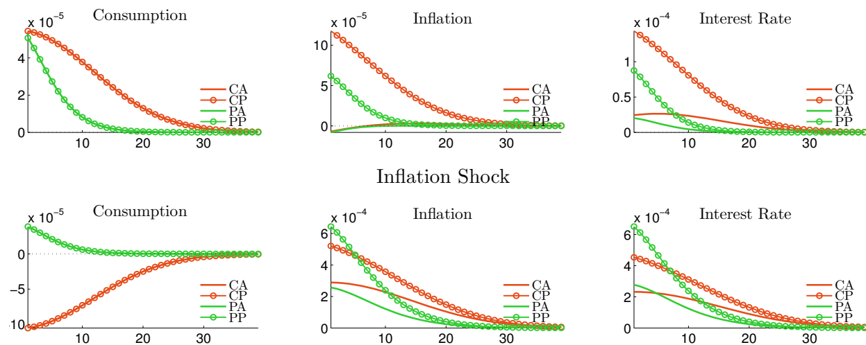
Figure A-2: Impulse Response Function
