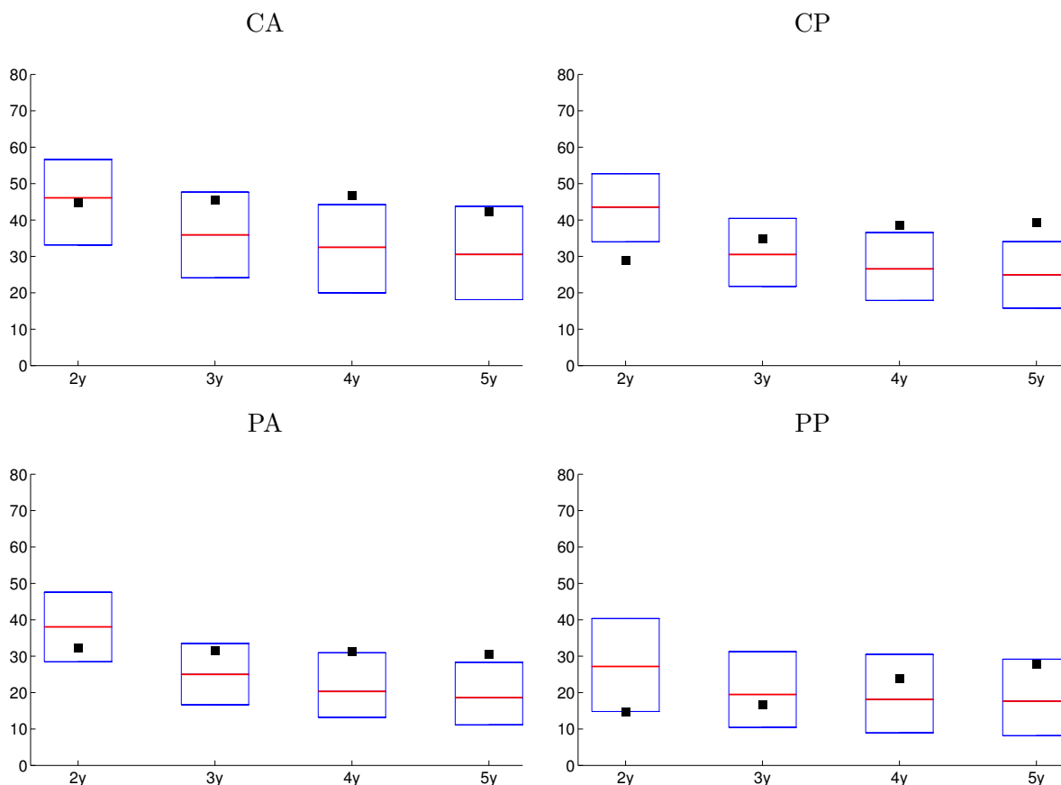
Figure 7: Excess Bond Return Predictability Regression by Cochrane and Piazzesi (2005)
