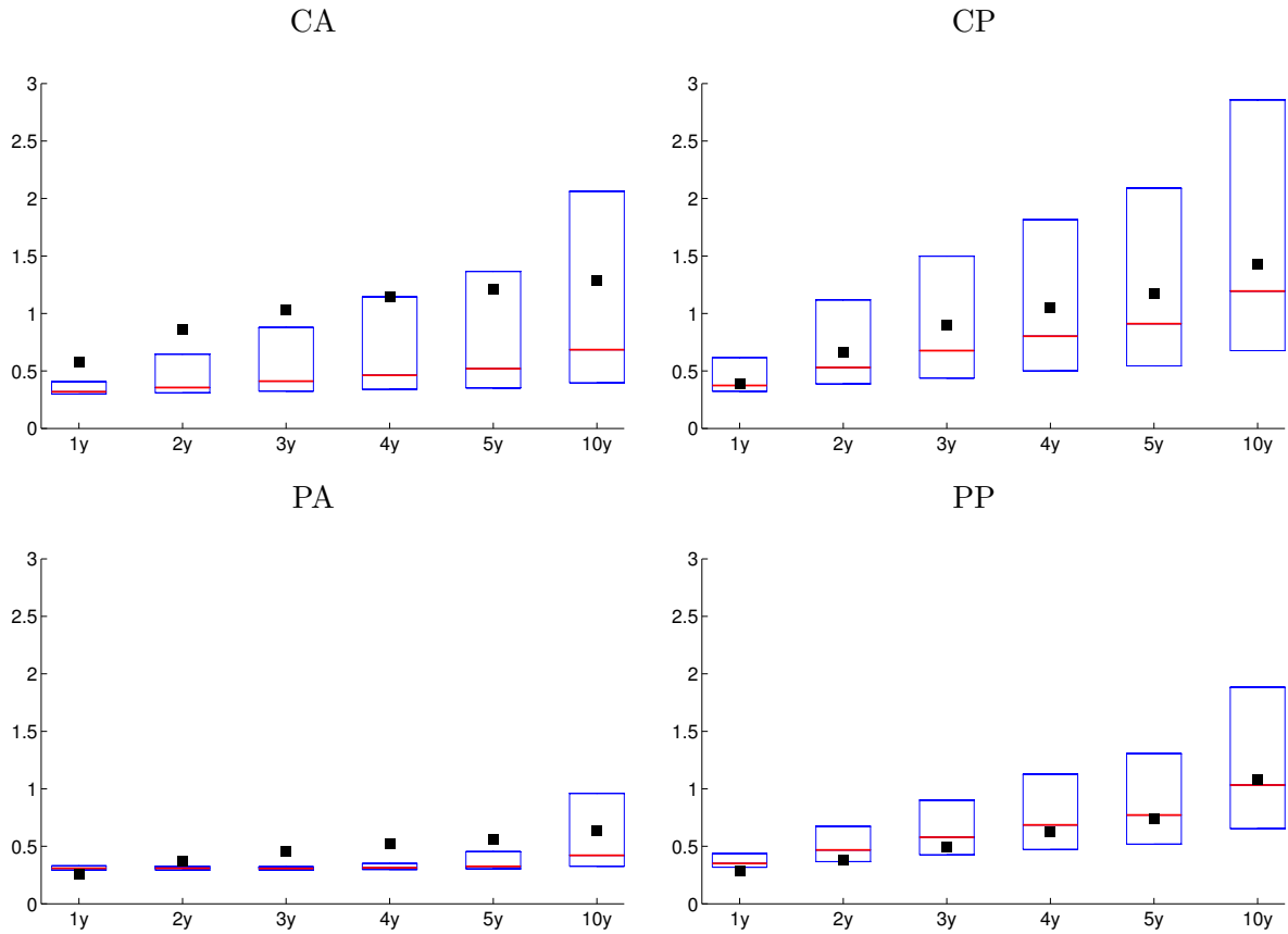
Figure A-6: Model-Generated Yield Spread: Unconditional Standard Deviation
