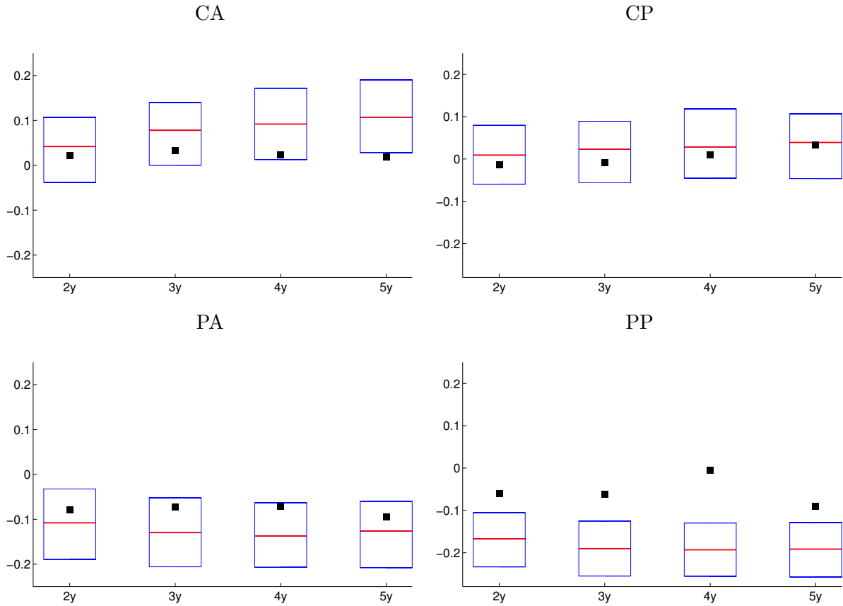
Figure 9: Stock-Bond Return Correlation
