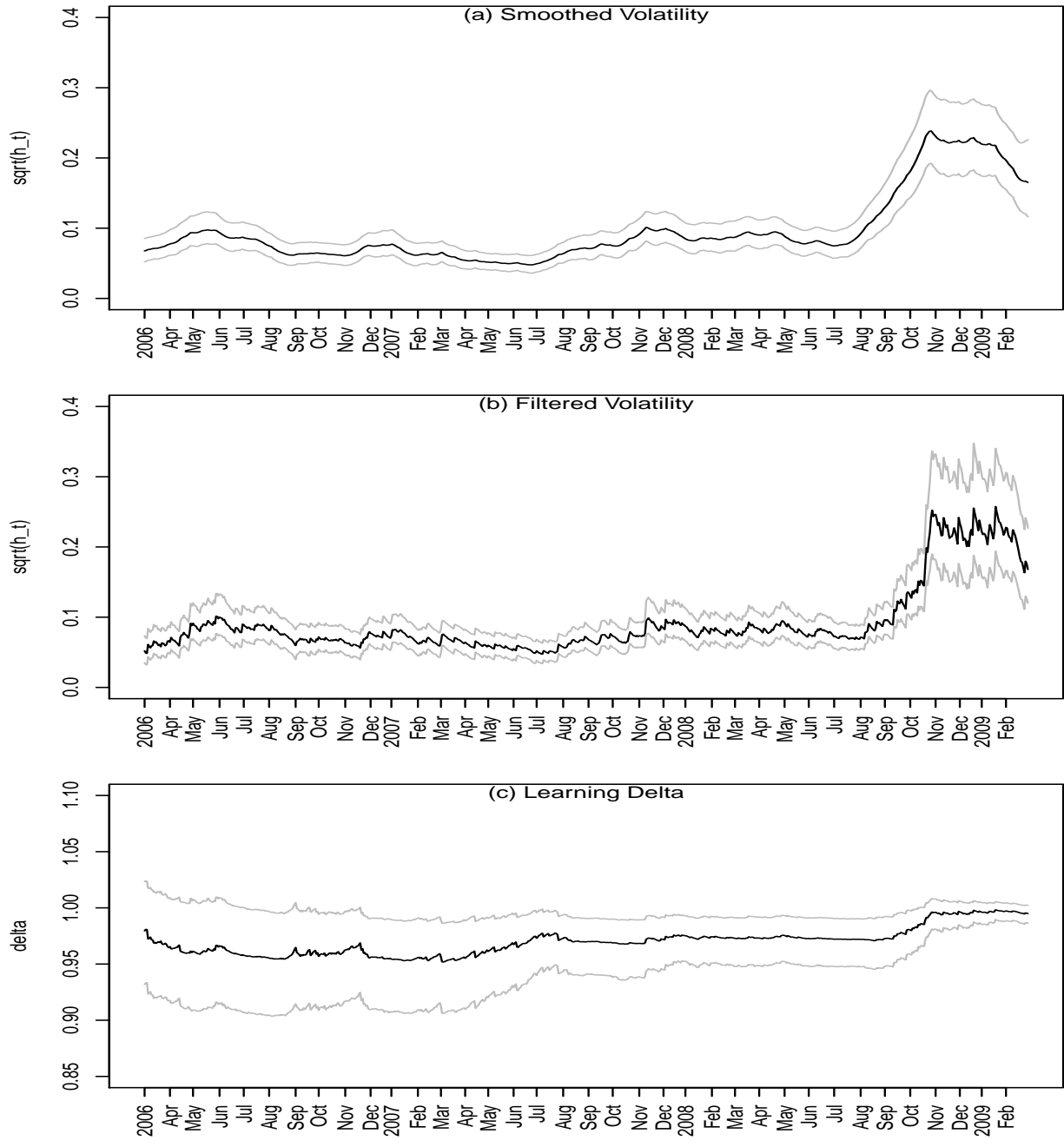
Figure 6: Smoothed \sqrt{h_t}|R^T , filtered \sqrt{h_t}|R^t , learning \delta|R^t SV model, £/$, Jan. 2, 2006 to Feb. 26, 2009, Mean and 5%, 95% quantiles.
